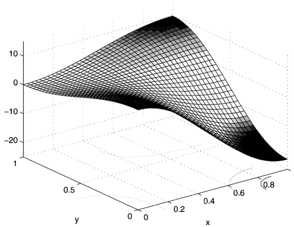
FIGURE 2 The regularized solution with \varepsilon = 10^{-2} .
