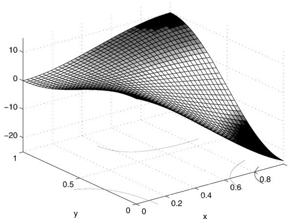
FIGURE 3 The exact solution.
