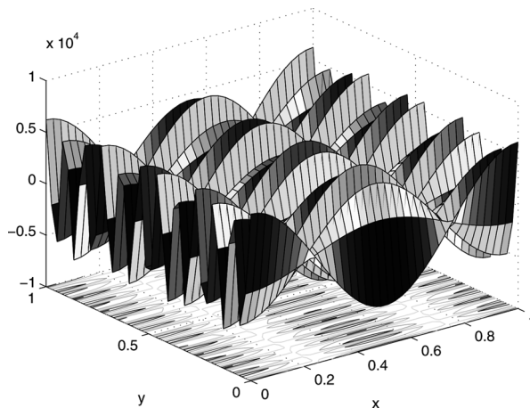
FIGURE 1 The disturbed solution with \varepsilon = 10^{-2} .
